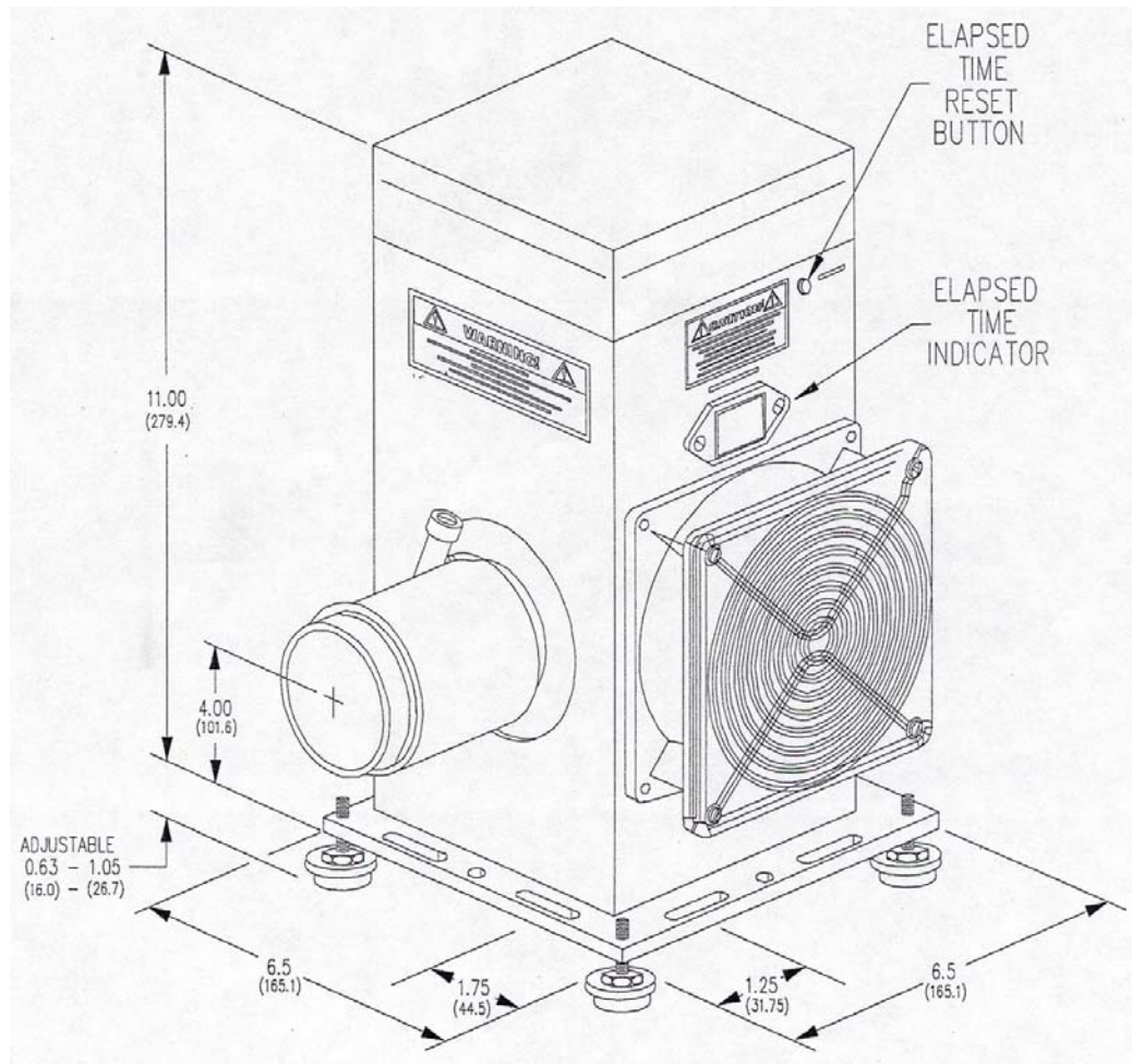
Figure 2 Dimensional Diagram
